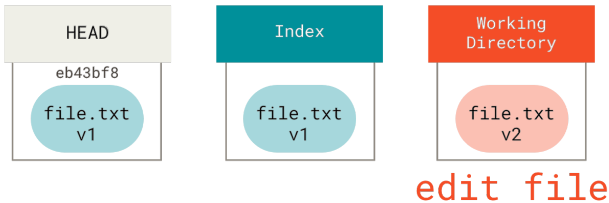
Figure 141. Git repository with changed file in the working directory
